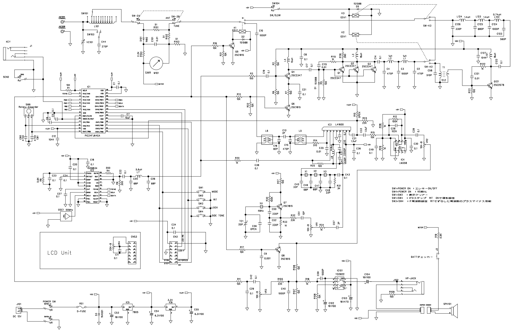
KEM TRX7 LITE QRP Transceiver + 5W Power Amp.
